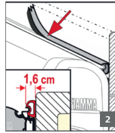
Rain Guard S
